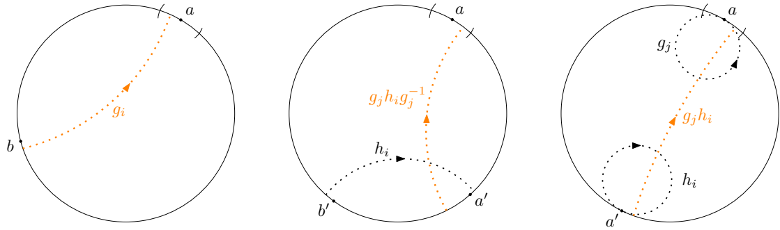
FIGURE 2. An illustration of Lemma 2.19. From left to right: the case when a \neq b , the case when a' \neq b' , and the case when a = b and a' = b' .
