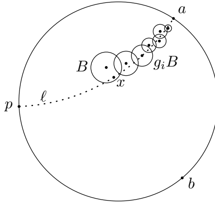
FIGURE 5. Illustration of the proof of Theorem 3.4
