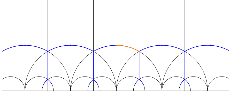
FIGURE 1. The tiling of the upper half plane corresponding to the action of \mathrm{SL}_2(\mathbb{Z}) . The tree in blue is preserved, with fundamental domain in orange.
