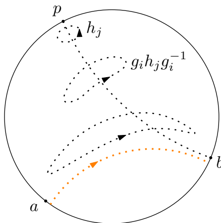
FIGURE 4. Illustration of Proposition 2.25. Conjugating the h_j by g_i distorts them enough to force them to eventually be loxodromic.
