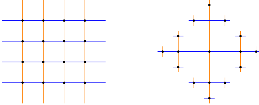
FIGURE 1. The Cayley graphs \Gamma(\mathbb{Z}^2, \{(1,0), (0,1)\}) and \Gamma(F(a,b), \{a,b\}) .
