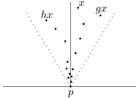
FIGURE 3. A conical limit point p in \partial \mathbb{H}^2 , in the upper half plane model. The dashed lines bound a uniform neighbourhood of the vertical geodesic line that tends to p , and the dots are G -translates of a point x \in \mathbb{H}^2 .
